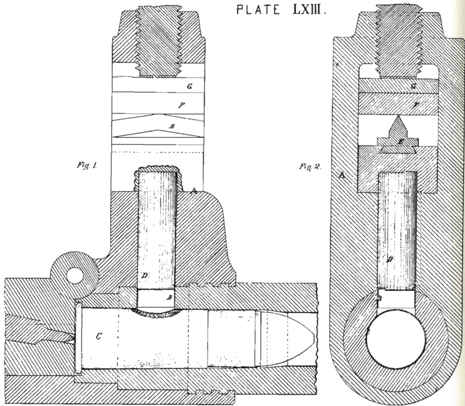
PRESSURE S. SERVICE GUN AND CARTRIDGE.
