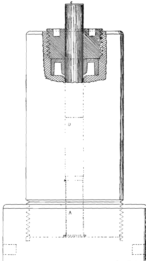
HYDROSTATIC PRESS.
