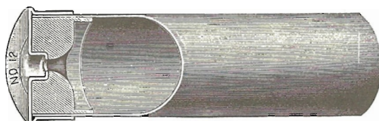
Paper Shot Shell, cut open, showing Improved Conical Base.
