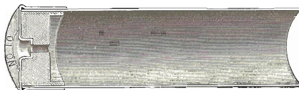
Paper Shot Shell, cut open, showing Old Style Base.
